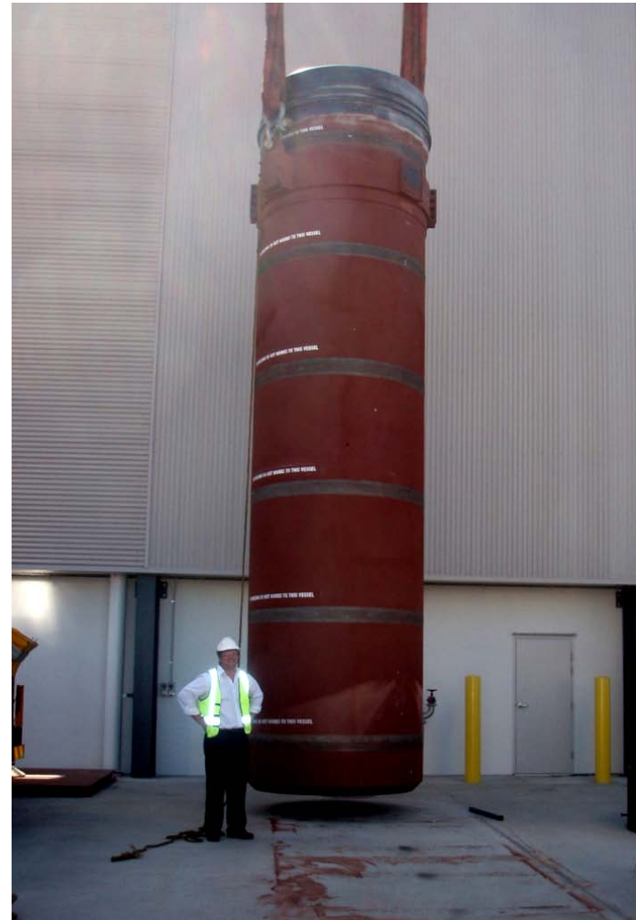
Paul Riordan GM of Matrix Offshore Services & Engineering Division Standing next to Matrix's new 5000msw rated deepwater Chamber – weighing in at 63,000kg. The Chamber was designed and manufactured by Paul's team.
